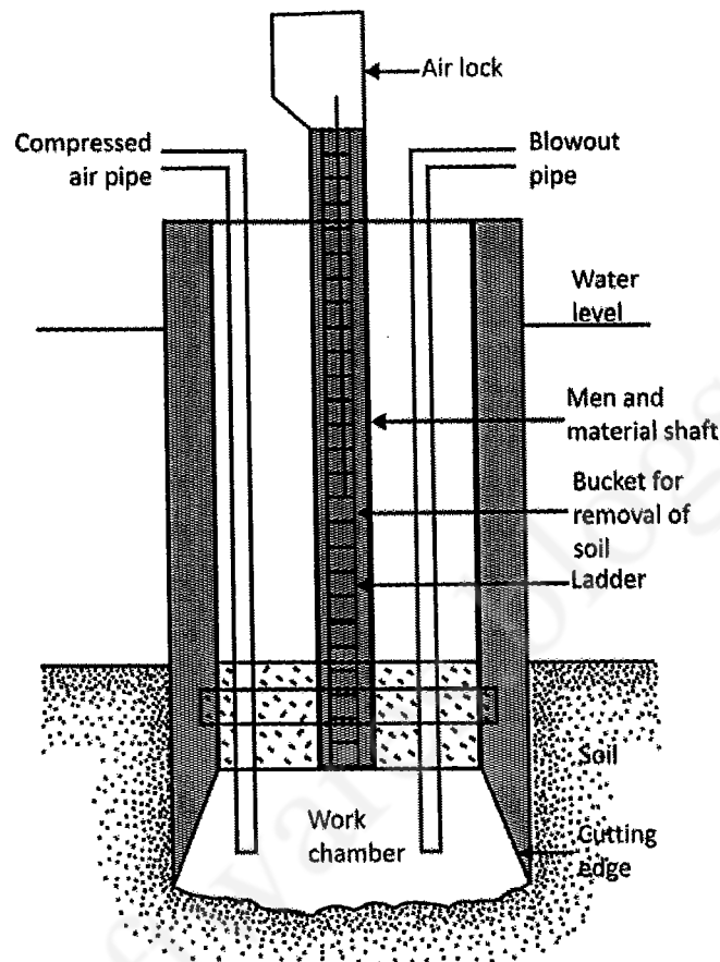
Figure 9.32 Pneumatic caisson
